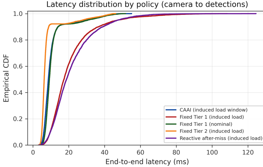
Fig. 7: Schematic reporting format: end-to-end latency CDF for the instrumented perception path, with one empirical step-CDF curve per condition. Each curve should pool all samples collected under that condition. This schematic illustrates the required format; measured curves from a physical deployment would replace it.
