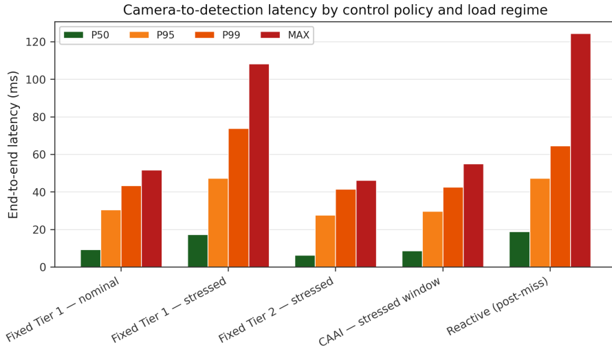
Fig. 8: Schematic reporting format: end-to-end latency summary by condition. Bars show p50, p95, p99, and max derived from measured samples. The start/stop timestamps used to compute camera→detection latency must be specified in the experiment setup text. This schematic illustrates the required format; measured bars from a physical deployment would replace it.
