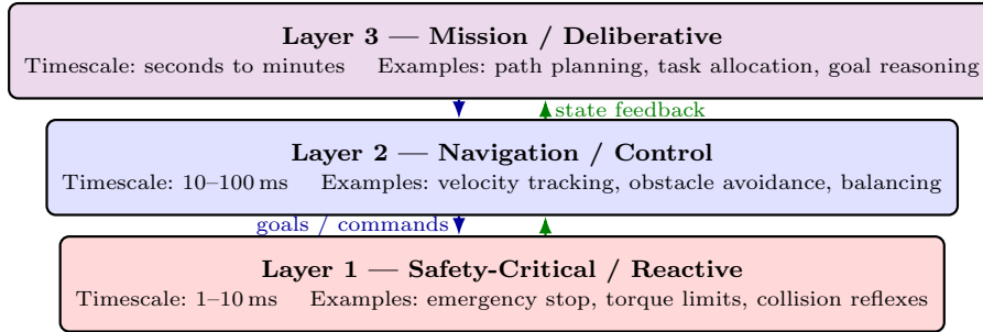
Fig. 4: Three-layer hierarchical control architecture. Layer 1 (red) provides hard real-time guarantees: it responds within 1–10 ms regardless of the higher layers. Goals flow downward (solid); state feedback flows upward (dashed). If a higher layer crashes, lower layers continue to guarantee basic safety. (Author-created figure.)
