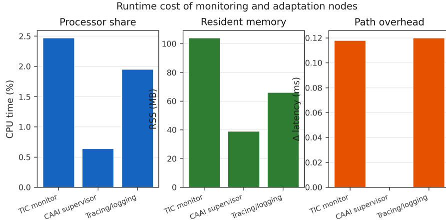
Fig. 9: Schematic reporting format: monitoring overhead per component (CPU share %, RSS memory in MB, and added latency \Delta ms as defined in Table 12). This schematic illustrates the required format; measured values from the instrumented prototype would replace it.
